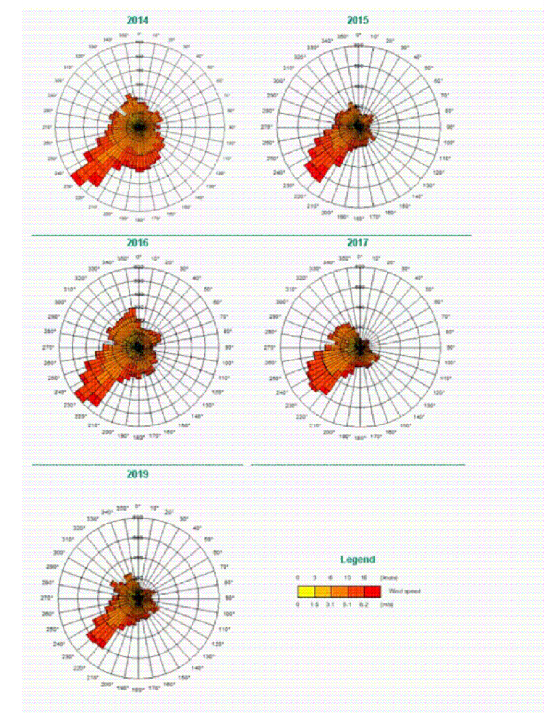
WIND ROSE STUDY FOR STANSTED AIRPORT
